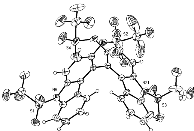
Figure 2. ORTEP drawing of the crystal structure of 17 .
