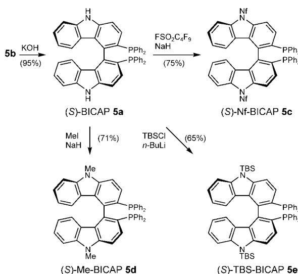
Scheme 3. Creation of the BICAP family.
