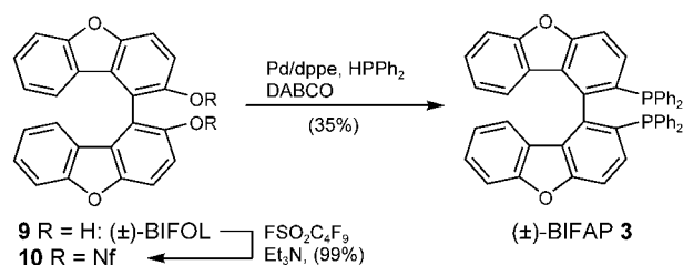
Scheme 1. Synthesis of BIFAP using HPPH 2 .
