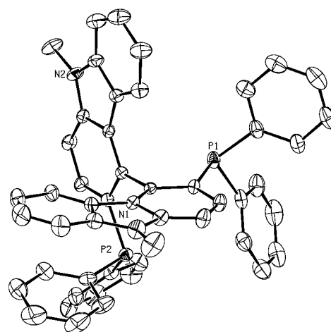
Figure 3. ORTEP drawing of the crystal structure of ( S )-Me-BICAP 5d .
