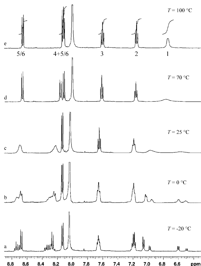
Figure 1. ^1\text{H} NMR spectra of 17 at different temperatures (in \text{DMF-d}_7 ).
