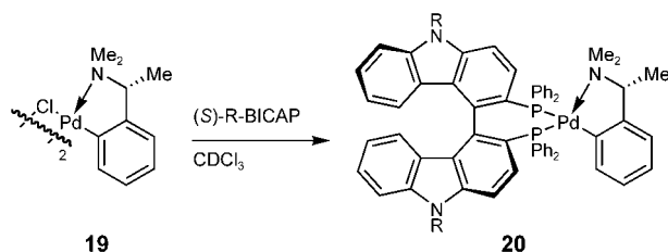
Scheme 4. Checking the enantiopurity of the BICAP ligands.
