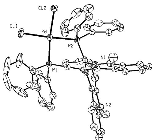
Figure 4. ORTEP drawing of the crystal structure of [( S )-Me-BICAP]PdCl 2 18 .
