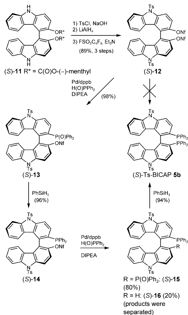
Scheme 2. Synthesis of Ts-BICAP.
